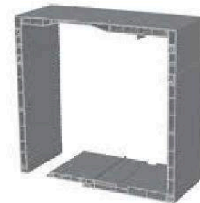
Caisson PVC 245 x 255 mm (se compose de 7 parties)
